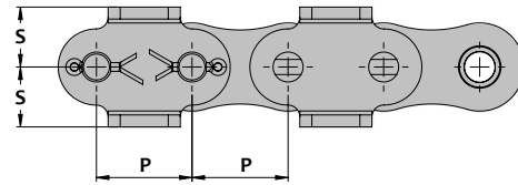
KK-1 Attachment
