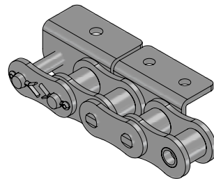
WA-1 or WA-2 Wide Contour Bent Lug One Side One Hole (WA-1) Two Holes (WA-2)
