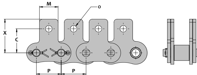
SK-1 Attachment
