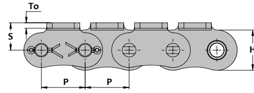
K-1 Attachment
