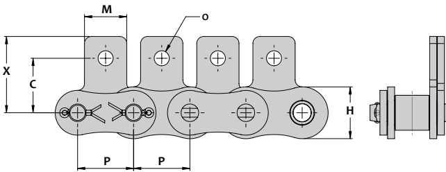
SA-1 Attachment
