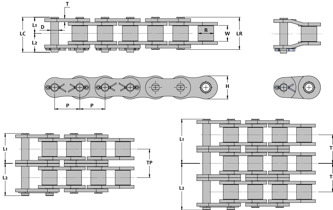
Chain Dimensions - Single Strand
