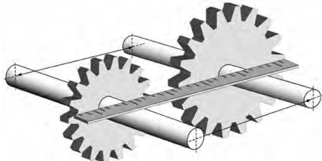
Sprocket Alignment
