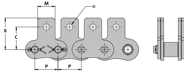
SK-1 Attachment
