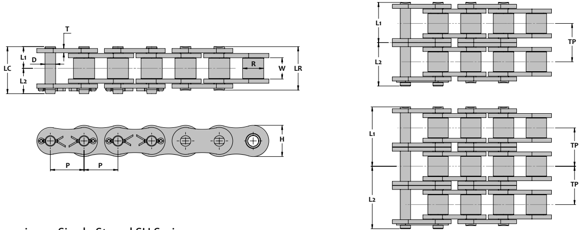
Chain Dimensions - Single Strand SU Series
