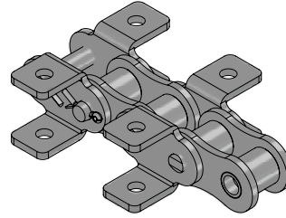
KK-1 Bent Double Lug Up and Down Two Sides - One Hole
