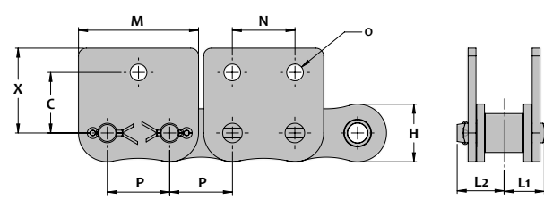
WSK-1/WSK-2 Attachment
