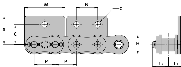
WSA-1/WSA-2 Attachment
