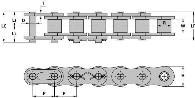
Chain Dimensions - Single Strand
